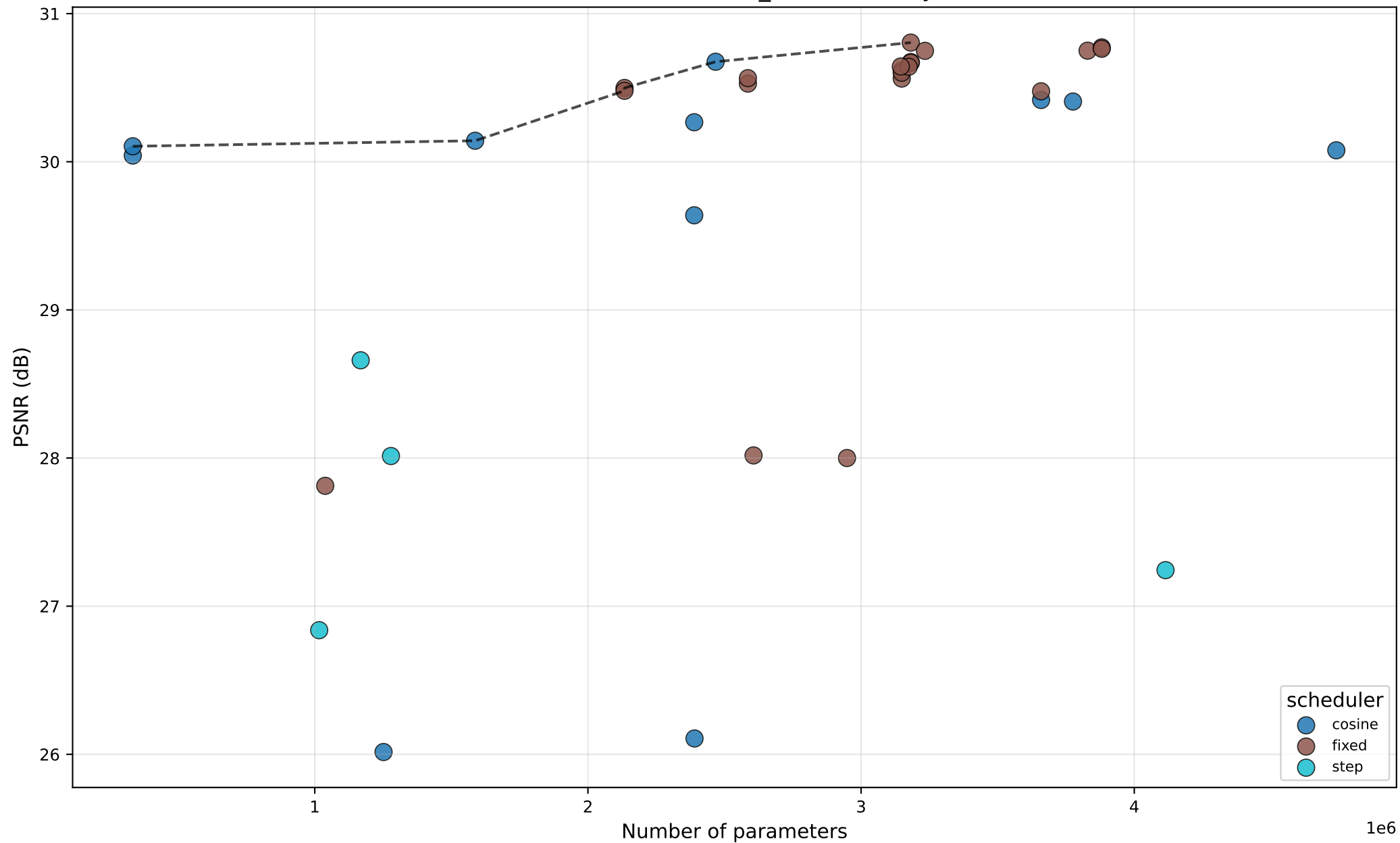
PSNR vs #Params — DHTCUN_baseline — by scheduler
